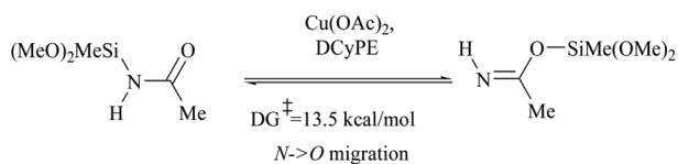
Scheme 30 DFT calculations: Cu catalyzed interconversion of N -silyl and O -silyl imidate forms.
