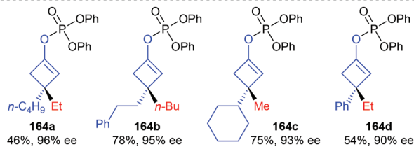
Scheme 46 Enantioselective 1,4-addition/trapping reaction of 3-substituted cyclobutenones.
