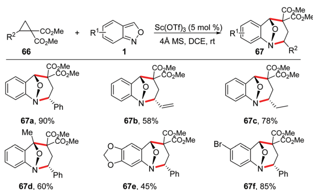
Scheme 23 [4 + 3]-annulation reaction between cyclopropane 1,1-diester and anthranils.
