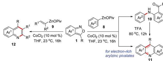
Scheme 4 Co-Catalysed amination of organozinc pivalates with anthranils.
