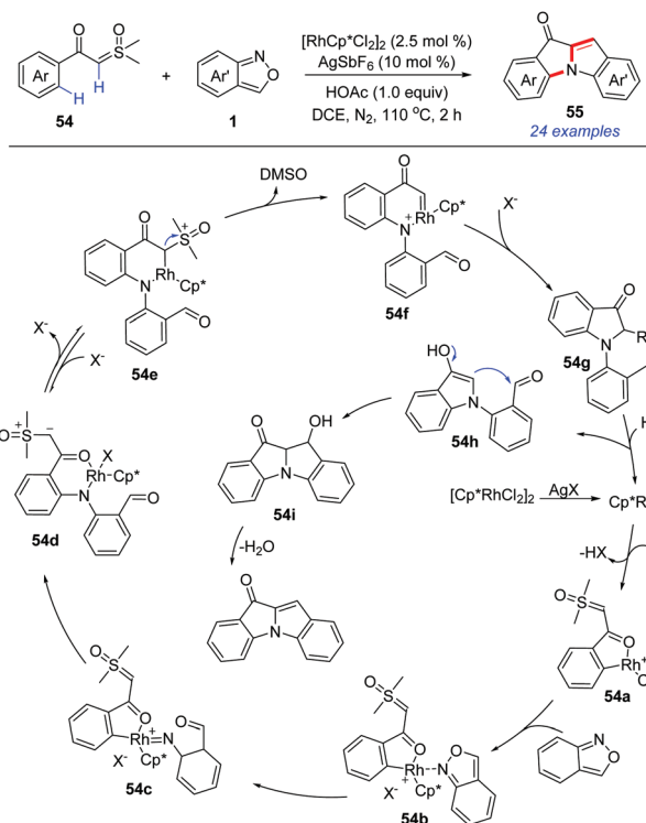
Scheme 19 Rh-Catalysed C–H annulation of \alpha -royl sulfoxonium ylides with anthranils.
