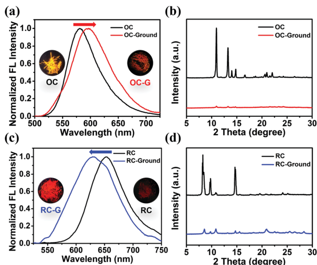
Fig. 6 (a) Normalized FL spectra ( \lambda_{\text{ex}} = 400 nm) and (b) PXRD patterns of OC before and after being ground. (c) Normalized FL spectra ( \lambda_{\text{ex}} = 400 nm) and (d) PXRD patterns of RC before and after being ground.
