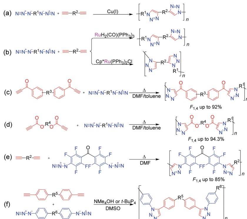
Fig. 6 AACPs: (a) CuAACP, (b) RuAACP, and (c) MFCP of arylacetylene and azide monomers; (d) MFCP of propiolate and azide monomers; (e) MFCP of 4,4'-diazidoperfluorobenzophenone and alkyne monomers; and (f) organobase-mediated AACPs.
