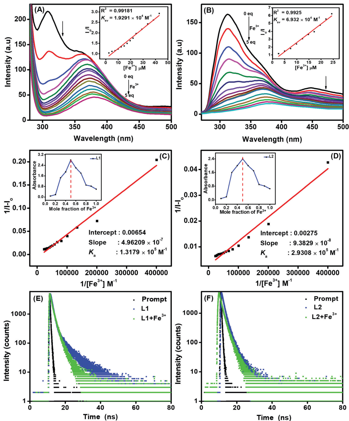
Fig. 5 Fluorescence titration spectra with 1 \times 10^{-5} \text{ M} (A) L1 and L2 (B) in THF-H 2 O (10%:90% and 40%:60%) upon successive addition of Fe 3+ ions (0 to 5 equivalents) ( \lambda_{\text{ex}} = 255 \text{ nm} ). Insets: K_{sv} plots for L1 and L2 . B-H plots of (C) L1 and (D) L2 using 1:1 stoichiometry for the associations of L1 and L2 with Fe 3+ ions. Insets: Job's plot for the complexation of L1 and L2 with Fe 3+ ions plotted using absorbance changes by the mole fraction method. Fluorescence lifetime decay plots of L1 (E) and L2 (F) in the absence and presence of Fe 3+ ion.
