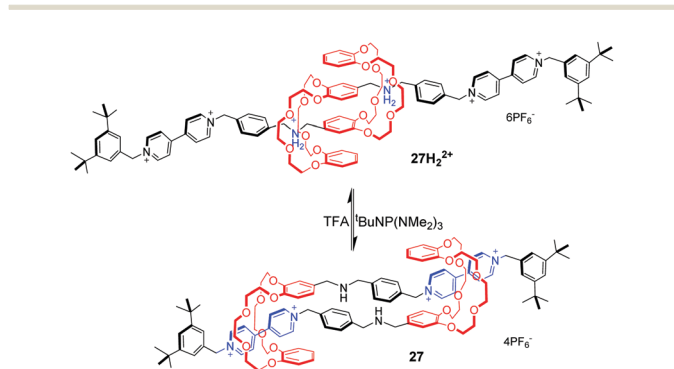
Fig. 27 pH-Actuated [c2]daisy chain 27 .
