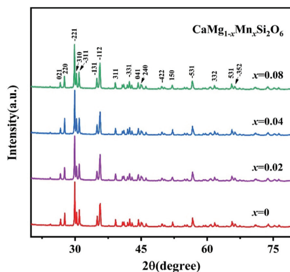
Fig. 4 The XRD patterns of \text{CaMg}_{1-x}\text{Mn}_x\text{Si}_2\text{O}_6 ( x = 0-0.08 ) ceramics sintered at 1300 °C (reprinted with permission from ref. 102. Copyright 2019 Elsevier).
