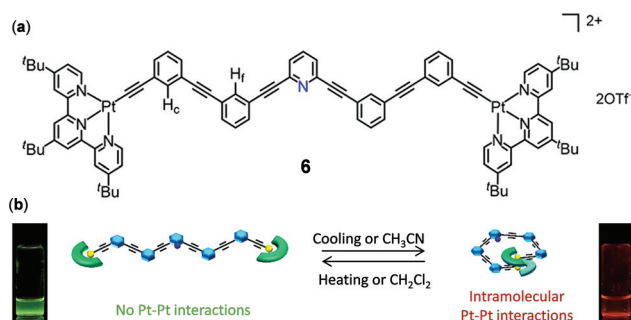
Fig. 5 (a) Molecular structure of Pt(II) complex 6. (b) Schematic diagram showing the reversible helix–coil molecular configuration transformation regulated by solvents and temperature. Reprinted with permission from ref. 93. Copyright 2019 American Chemical Society.
