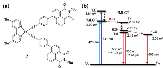
Fig. 6 (a) Molecular structure of Pt(II) complex 7. (b) Simplified Jablonski diagram showing the energy levels of 7. BZN = benzonitrile. Tol = toluene. Reprinted with permission from ref. 96. Copyright 2019 American Chemical Society.
