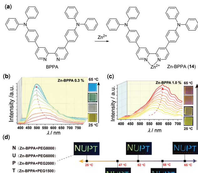
Fig. 13 (a) Chemical structures of BPPA and Zn(II) complex 14 . (b and c) Temperature-dependent emission spectral and color change of PEG8000 containing (b) 0.3 wt% and (c) 1.0 wt% of 14 within the temperature range of 25–65 °C. (d) Photographs displaying thermochromic luminescent NUPT patterns at different temperatures. The letters “N, U, P, and T” were written on a glass substrate using 14 /PEG8000, 14 /PEG6000, 14 /PEG2000 and 14 /PEG1500 composites containing 0.3, 0.3, 0.2, and 0.2 wt% of 14 , respectively. Reprinted with permission from ref. 102. Copyright 2020 WILEY-VCH.
