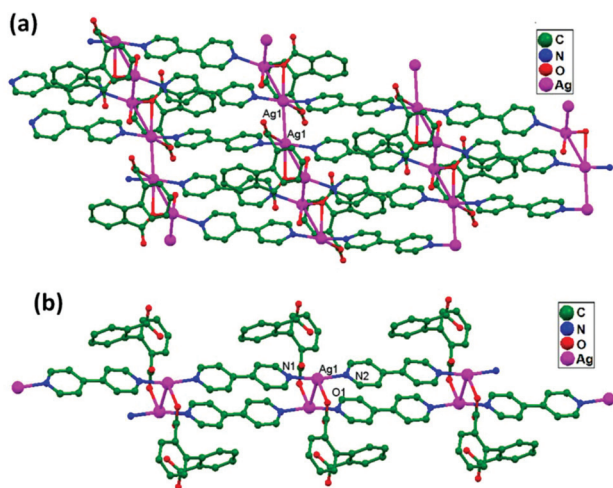
Fig. 37 The compounds (a) \text{Ag}_2(\text{bpy})_{1.5}(\text{dpa})(\text{H}_2\text{O}) , 59 , and (b) \alpha\text{-}[\text{Ag}(\text{4,4}'\text{-bpy})]_3(\text{Hdpa}) , 60 , showing ligand-unsupported argentophilic interactions.
