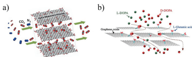
Fig. 2 (a) Schematic illustration of the facilitated transport of CO_2 through the GO membrane via the chemical interaction between CO_2 molecules and the oxygen-containing functional groups on the surface of the GO layers. 43 (b) Chiral separation of D- and L-DOPA by the L-glutamic acid functionalized GO membrane through the chiral interaction between L-glutamic acid and D-DOPA. 44 Copyright, 2014 Wiley-VCH and 2016 Elsevier.
