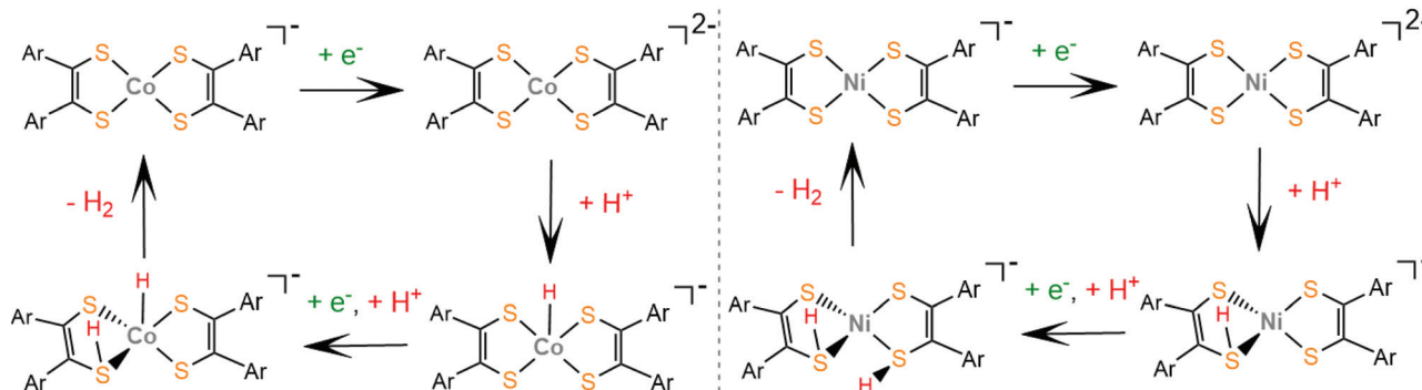
Scheme 11 (a) Structures of aryl-benzene complexes. (b) Proposed mechanisms catalysed by complexes 17a (left) and 18a (right).
