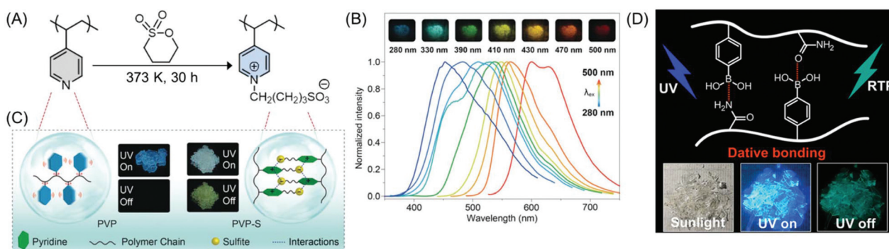
Fig. 12 (A) Synthetic route to an amorphous PVP-S polymer. (B) Phosphorescence spectra of PVP-S acquired at 77 K at various excitation wavelengths. Inset shows the afterglow multicolor phosphorescence emission on excitation with a wide range of wavelengths from 280 to 500 nm at 77 K. (C) Schematic illustration of ionization-induced ultralong phosphorescence of PVP-S. Reprinted with permission from ref. 75. Copyright (2019), WILEY-VCH. (D) Graphical representation of the RTP polymer involving boron–nitrogen dative bonds and their fluorescence images under sunlight and UV “on–off” conditions. Reprinted with permission from ref. 76. Copyright (2020), American Chemical Society.
