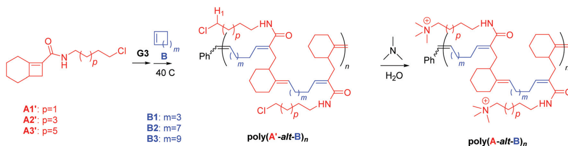
Scheme 1 Synthesis of intermediate copolymers poly(A'- alt -B) n via AROMP and cationic copolymers poly(A s - alt -B) n via post-polymerization functionalization.
