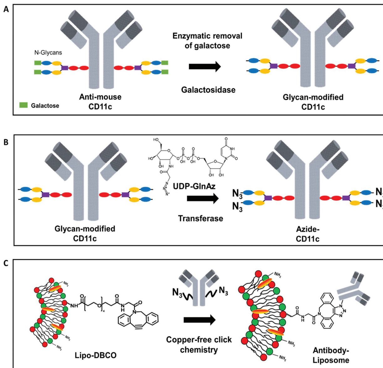
Fig. 3 Antibody functionalization and attachment to surface-modified liposomes. (A) Enzymatic removal of galactose from the CD11c-antibody with galactosidase. (B) Site-specific, enzymatic attachment of an azide functionality using UDP-N-azidoacetylgalactosamine (UDP-GlnAz) to the sugar residues on the Fc-part of the CD11c-antibody (C) bio-orthogonal copper-free click reaction to attach the azide-modified antibody on the DBCO-modified liposome surface.
