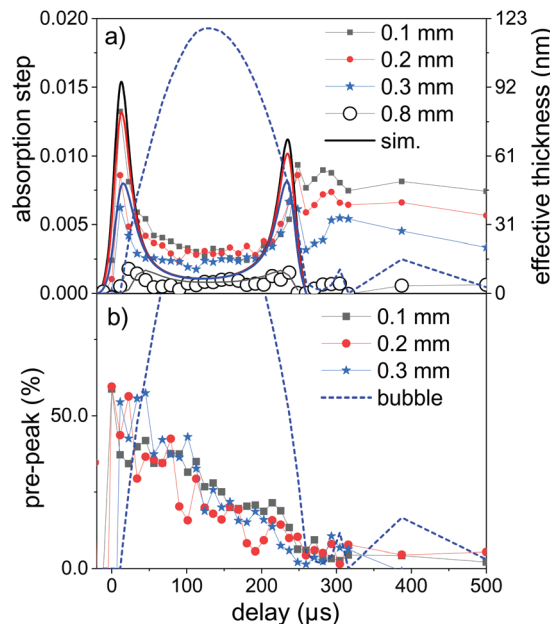
Fig. 4 (a) Time dependence of the step height at the Zn K edge as a measure for the total intersected material by the X-ray beam at several distances above the target (symbols). The lines are model calculations assuming a homogeneous filling of the bubble with a fixed amount of material. (b) Time dependence of the ratio of the pre-peak to metallic Zn absorption as a measure for the relative atomic content at several distances. The dashed line in each sub-figure represents the X-ray transmission change due to bubble formation.
