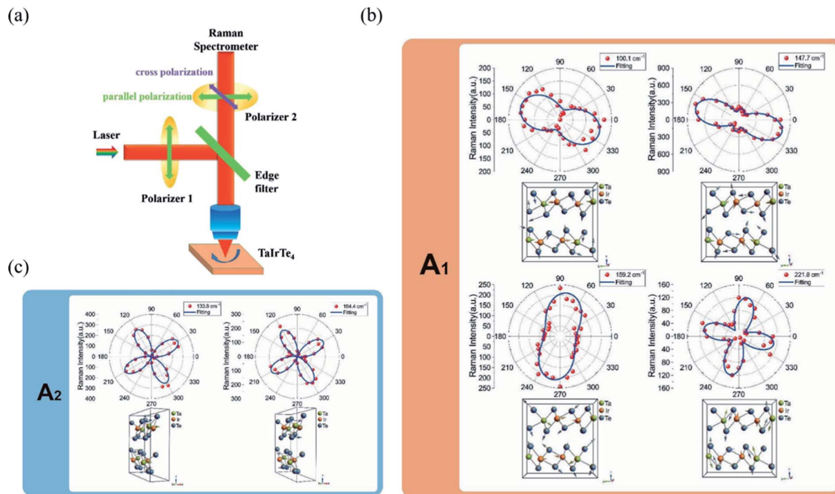
Fig. 8 (a) Schematic of the angle-resolved polarized Raman spectroscopy of TaIrTe 4 samples. Raman intensities of (b) A 1 and (c) A 2 modes as a function of the sample rotation angle and the corresponding phonon modes in the atomic view. The scattered dots are the experimental data and the solid lines are the fitting curves. Reproduced from ref. 49 with permission from Wiley-VCH.
