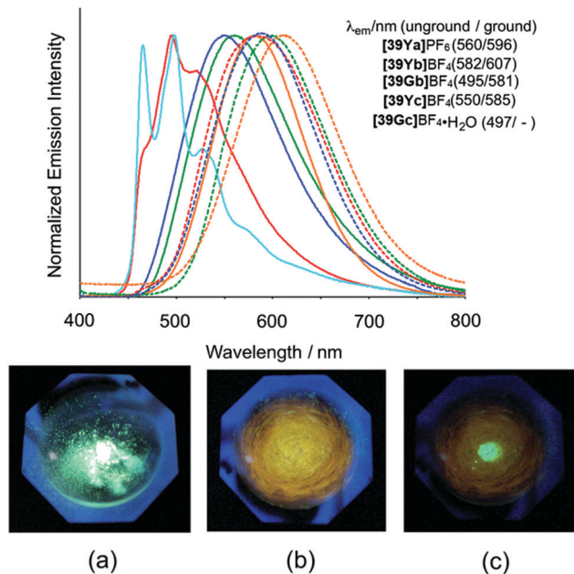
Fig. 15 Top: Normalized emission spectra of the Pt II based complexes in the solid state at 295 K ( \lambda_{\text{ex}} = 365 nm). Solid and dashed lines correspond to the spectra of unground and ground samples, respectively. Bottom: Photographic images of [39Gb]BF 4 in response to mechanical grinding under UV light irradiation (365 nm): (a) unground sample, (b) completely ground sample, (c) ground sample with a drop of acetonitrile. Reprinted with permission from ref. 57. Copyright 2014 Royal Society of Chemistry.
