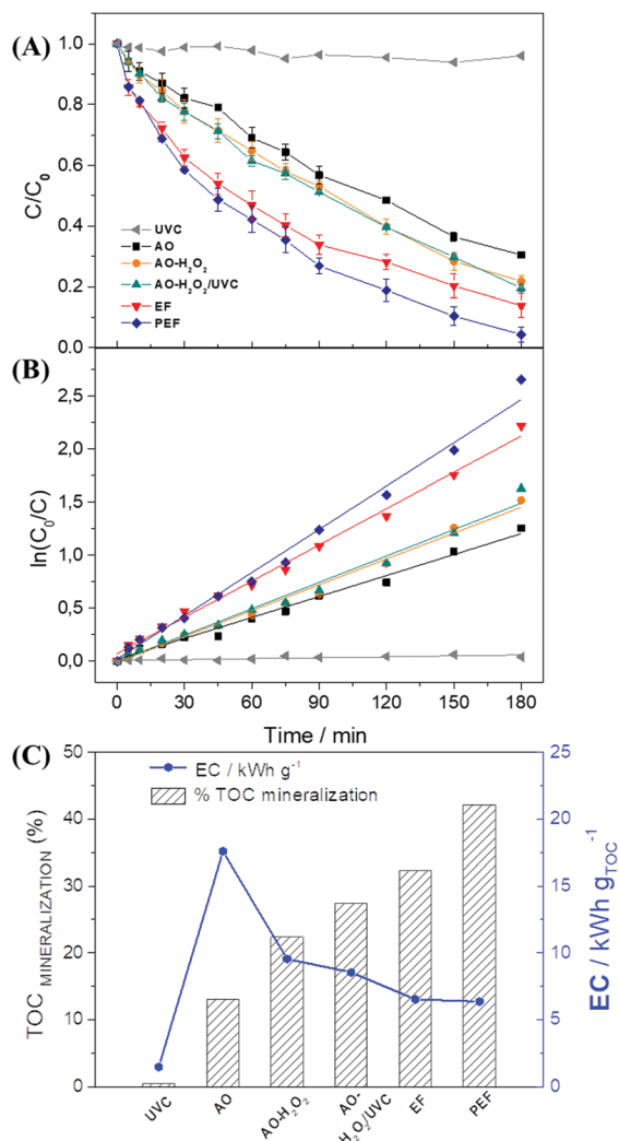
Fig. 5 (A) Effect of different AEOPs on PRM degradation in 180 min of experiment at j = 75\ mA\ cm^{-2} using the 1.0% NQE modified GDE with 0.1\ mol\ L^{-1}\ K_2SO_4 under pH 2 and 0.2 bar of O_2 flow; (B) analysis of the pseudo-first order kinetics; and (C) comparison between the TOC mineralization and energy consumption in each system.
