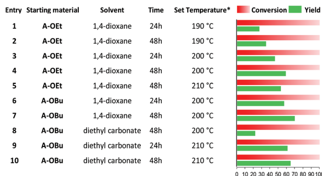
Fig. 6 Catalytic dehydrogenative decarbonylation A-OEt or A-OBu to B-OEt or B-OBu. Reaction conditions: 15 mg substrate, [\text{Ir}(\text{cod})\text{Cl}]_2 5 mol%, 4 : 2 : 1 LiCl : rac -BINAP : [\text{Ir}(\text{cod})\text{Cl}]_2 , as catalyst; 190–210 °C in 1 mL solvent. Yield and conversion were determined by GC-FID using n -decane as an external standard; *Set temperature of the heating block; the measured corresponding inside temperature is shown in Table S1.†
