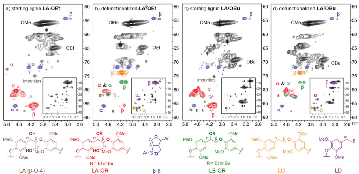
Fig. 8 2D-HSQC NMR spectra (600 MHz, CDCl 3 ) of the linkage region of (a) \alpha -ethoxylated lignin (starting lignin), (b) defunctionalized \alpha -ethoxylated lignin, (c) \alpha -butoxy lignin (starting lignin), and (d) defunctionalized \alpha -butoxy lignin; defunctionalized lignins were obtained by dehydrogenative decarbonylation; reaction conditions: 200 mg LA-OEt or LA-OBu with [\text{Ir}(\text{cod})\text{Cl}]_2 13.4 wt%, rac -BINAP 24.9 wt%, LiCl 3.4 wt% and a drop of water dissolved in 2.5 mL diethyl carbonate reacting at a set temperature of 205 °C for 48 hours.
