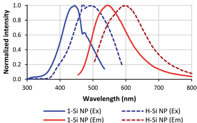
Fig. 6 Optical properties of Si NPs. Full lines: Si NPs passivated with 1; dashed lines: non-passivated Si NPs. Excitation spectra are shown in blue, emission spectra in red.
