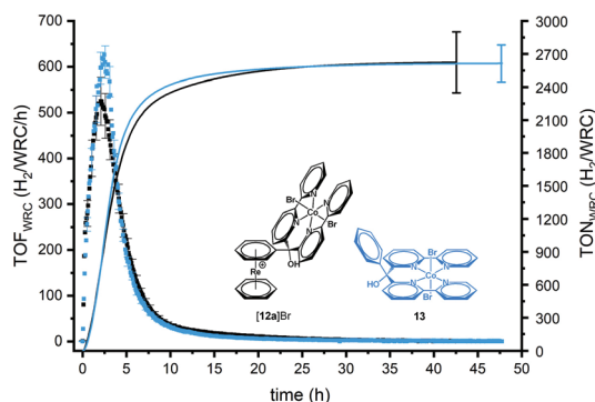
Fig. 4 Photocatalysis experiment with [\mathbf{12a}]^+\text{Br}^- in black and the parent catalyst 13 in blue. TOF (dots) ( \text{H}_2/\text{Co}/\text{h} ) and TON (lines) ( \text{H}_2/\text{Co} ) formed as a function of time for 5 \mu\text{M} catalyst. Experimental conditions: 10 mL solution, 0.5 mM [\text{Ru}(\text{bpy})_3]\text{Cl}_2 , 0.1 M NaAsc, 0.1 M TCEP, pH 5.0, 453 nm LED irradiation.
