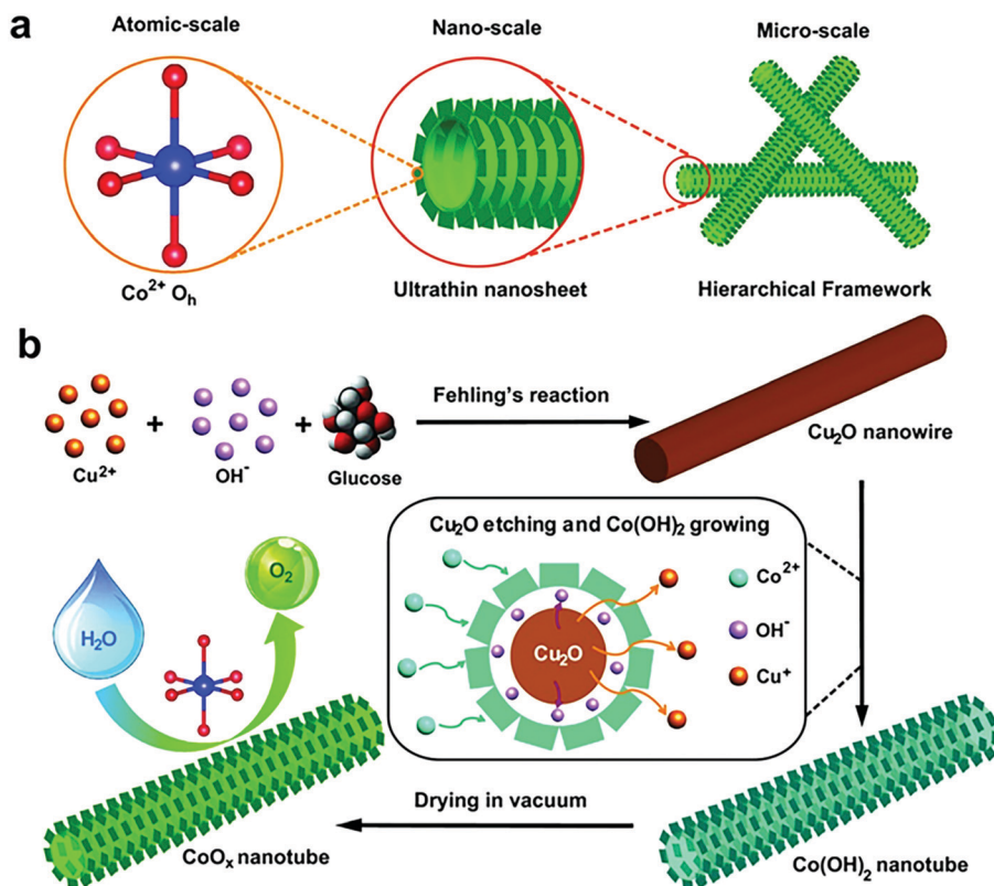
Fig. 7 (a) Schematic illustration of the design of hierarchical CoO x nanosheet/nanotube structures; (b) synthesis procedure of the hierarchical CoO x nanosheet/nanotube structures, including the in situ growth of Cu 2 O nanowire templates, etching of the nanowire templates and regrowth of ultrathin Co(OH) 2 nanosheets from the original nanowire template surface, and dehydration to form a CoO x nanosheet/nanotube structure. Reprinted with permission from ref. 258 (Creative Commons Attribution 4 International License).
