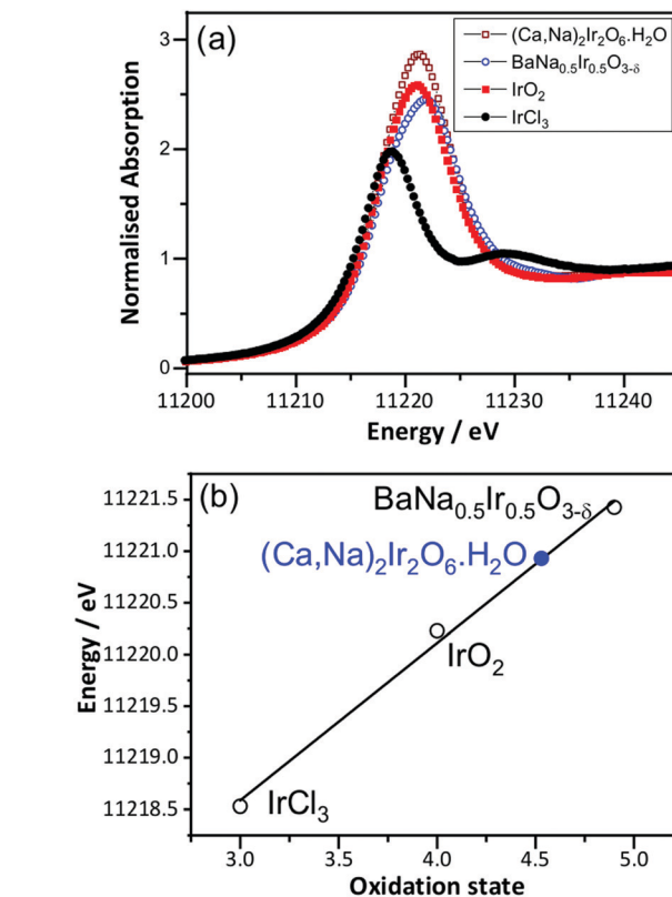
Fig. 2 (a) Room temperature Ir L_{\text{III}} -edge XANES spectra of (\text{Ca}_{0.70}\text{Na}_{0.24})_2\text{Ir}_2\text{O}_6 \cdot \text{H}_2\text{O} and reference materials and (b) oxidation state calibration graph, with the white line maximum used.
