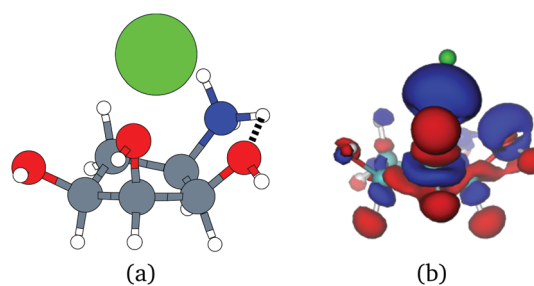
Fig. 4 (a) The molecular structure of the ligand with one zinc cation \text{Zn}^{2+} in the complex 3dx1. Hydrogen, carbon, nitrogen, oxygen, and zinc atoms are colored with white, gray, blue, red, and green, respectively. (b) The difference in the electronic probability density is plotted. Blue and red contours illustrate the gain and loss of the electronic probability density due to the embedding field.
