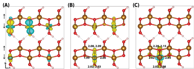
Fig. 4 Excess electron in lepidocrocite. (A) LUMO with asymmetry caused by degeneracy ( < 5 \text{ meV} ) between the top four levels. (B) Difference in spin density for vertical state, and (C) the relaxed state. The excess electron relaxes onto two parallel spin iron sites, with a positive increase in spin density caused by the addition of an anti-symmetric spin. Data for a 613 supercell of bulk lepidocrocite calculated with HSE06(18%)-D3. The ESI† contains an alternate view of the lepidocrocite electron polaron.
