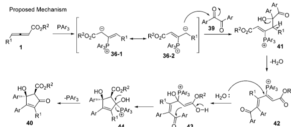
Scheme 12 Phosphine-mediated reaction of \gamma -alkyl allenates and diaryl 1,2-diones.
