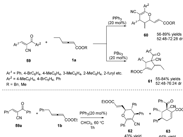
Scheme 18 Divergent phosphine-catalysed (2+4) or (3+2) cycloaddition reactions of oxadienes.
