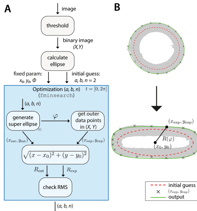
Fig. 2 Image-based estimation of \lambda_{\text{OP}} . (A) Schematic of displacement tracking algorithm. (B) Example of optimization result with the initial ellipse fit (dashed red), and the final super ellipse fit to the perimeter (green) for an undeformed (top) and deformed (bottom) sample. The sample contours are shown in gray.
