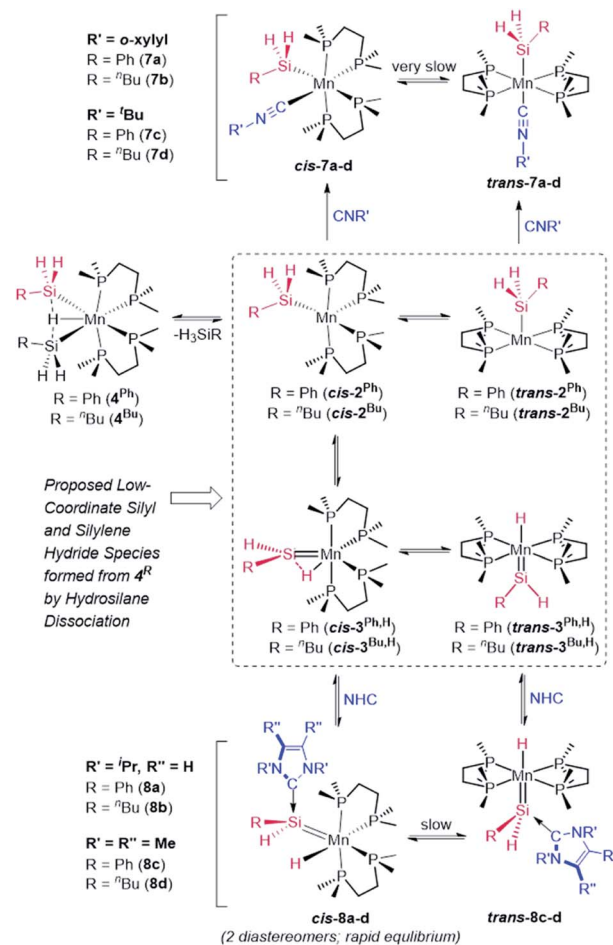
Scheme 5 Trapping of putative silyl (2 R ) and silylene hydride (3 R,H ) intermediates: synthesis of silyl isonitrile complexes [(dmpe) 2 Mn(SiH 2 R)(CNR')] ( 7a : \text{R} = \text{Ph} , \text{R}' = o\text{-xylyl} ; 7b : \text{R} = {}^n\text{Bu} , \text{R}' = o\text{-xylyl} ; 7c : \text{R} = \text{Ph} , \text{R}' = {}^t\text{Bu} ; 7d : \text{R} = {}^n\text{Bu} , \text{R}' = {}^t\text{Bu} ) and NHC-stabilized silylene hydride complexes [(dmpe) 2 MnH(=SiHR)(NHC)] ( 8a : NHC = i PrNHC, \text{R} = \text{Ph} ; 8b : NHC = i PrNHC, \text{R} = {}^n\text{Bu} ; 8c : NHC = Me NHC, \text{R} = \text{Ph} ; 8d : NHC = Me NHC, \text{R} = {}^n\text{Bu} ).
