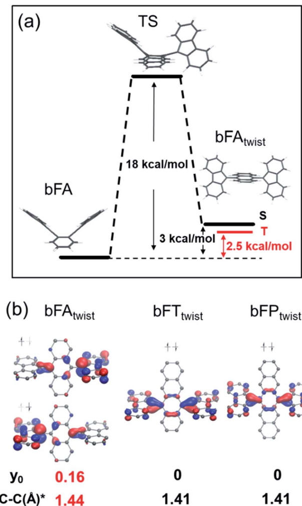
Fig. 5 (a) Energy diagram of \mathbf{bFA} with rotation of the fluorene moiety; (b) HOMOs of the fluorene twisted structure of \mathbf{bFA} ( \mathbf{bFA}_{\text{twist}} ), \mathbf{bFT} ( \mathbf{bFT}_{\text{twist}} ), and \mathbf{bFP} ( \mathbf{bFP}_{\text{twist}} ), with the y_0 value and bond length (*) of the C–C bond between fluorene and acenes.
