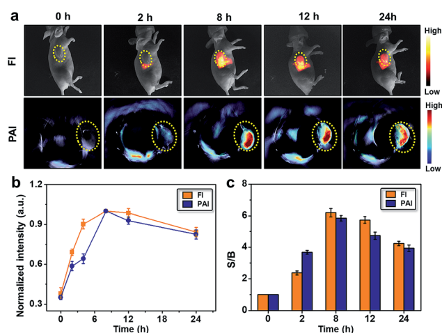
Fig. 4 In vivo multimodal images with SYL NPs. (a) In vivo NIR-II fluorescence (100 ms, 1\text{LP1000} , 82\text{ mW cm}^{-2} ) and PA images of 4T1 tumor-bearing mice at 0, 2, 8, 12, and 24 h after tail vein injection of SYL NPs. Yellow circles indicate tumor sites; (b) semi-quantified fluorescence and PA intensities; (c) time-dependence of the signal-to-background ratio (FI & PA) after intravenous injection.
