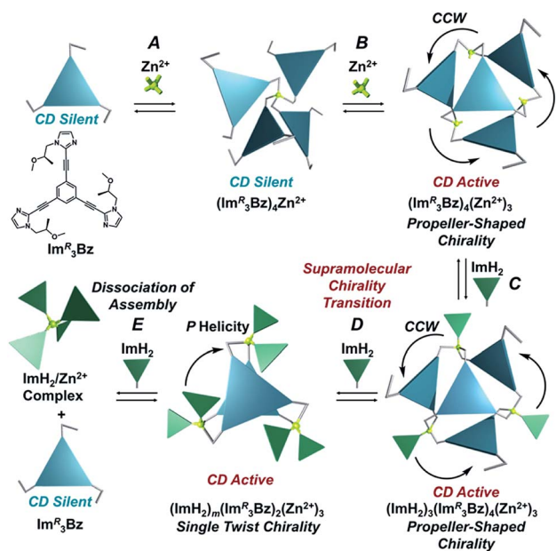
Scheme 3 Assembly formation of \text{Im}^R_3\text{Bz} with \text{Zn}^{2+} and \text{ImH}_2 .
