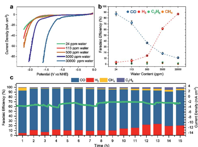
Fig. 3 Linear sweep voltammograms recorded at 5 \text{ mV s}^{-1} in MeCN with different water content and \text{CO}_2 purge (a), faradaic efficiencies of \text{CO}_2 reduction products in the gas phase at a constant potential of -1.8 V vs. NHE from MeCN with various amounts of water (b). Long term electrolysis for 15 h at -1.8 V vs. NHE with 24 ppm water including the observed faradaic efficiencies (c).
