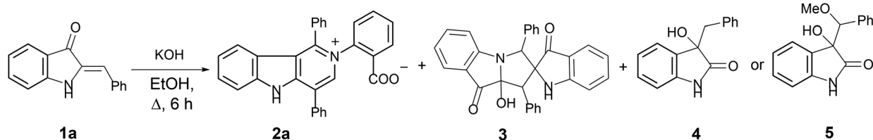
Scheme 1 Transformation of hemiindigo 1a in the alkaline conditions.
