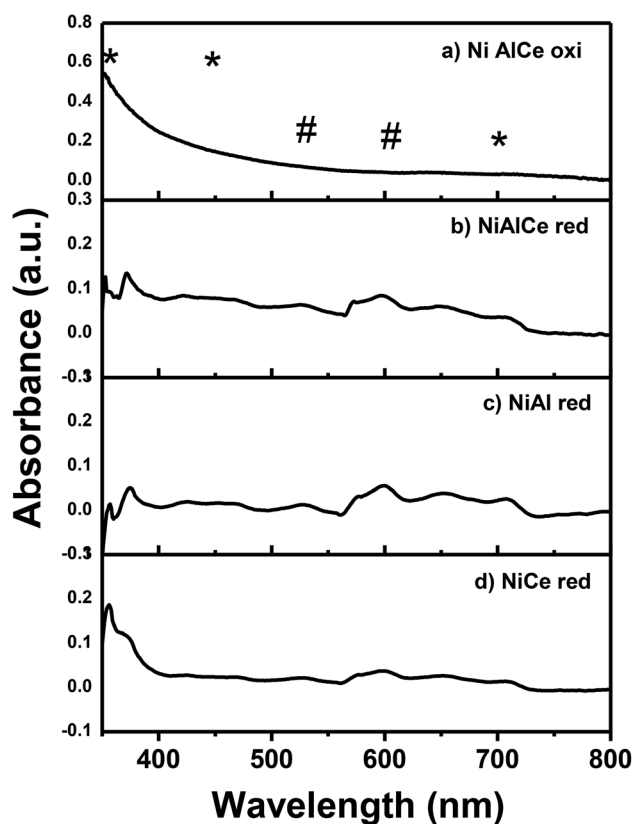
Fig. 6 Spectra UV-Vis for the calcined Ni supported catalyst: (a) and for the reduced Ni supported catalysts: (b), (c) and (d). Legend: (#) \text{Ni}^{+2}(\text{OH}) , (*) \text{Ni}^{+2}(\text{OH}) .
