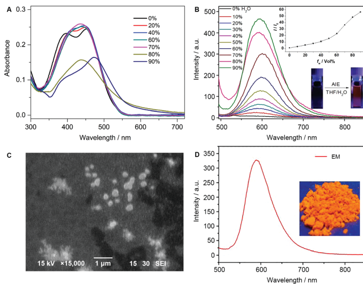
Fig. 2 Absorption and emission spectra: (A) absorption and (B) emission spectra of the AIEgen monomer EM ( 10 \mu\text{M} ) in \text{H}_2\text{O}/\text{THF} mixtures with different water fraction ( f_w ) from 0–90%, \lambda_{\text{ex}} = 460 \text{ nm} ; insets (B): plot of relative emission intensity against f_w and fluorescent images of EM ( f_w = 0 and 90%) under UV light illumination. (C) SEM image of nanoaggregates obtained from the EM suspension ( f_w = 90\% ). (D) Emission spectrum of EM in the solid state, \lambda_{\text{ex}} = 460 \text{ nm} ; inset: fluorescent image of the solid EM under UV light illumination.
