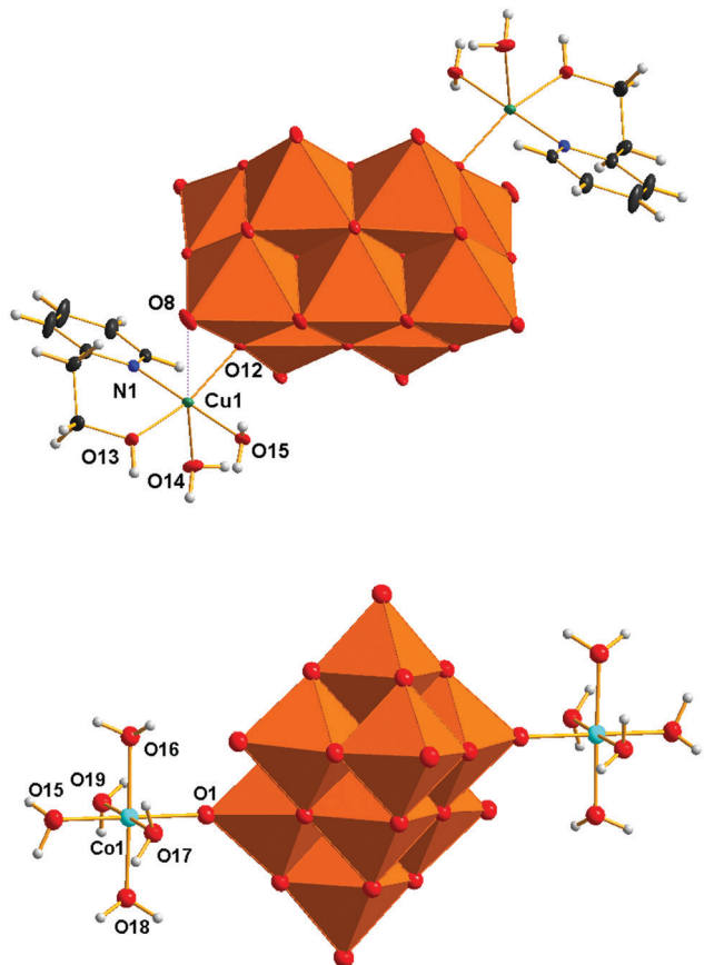
Fig. 1 Molecular structures of the anions [\{\text{Cu}(\text{H}_2\text{O})_2(2\text{-hep})\}_2\text{V}_{10}\text{O}_{28}]^{2-} ( \text{V}_{10}\text{Cu} ) and [\{\text{Co}(\text{H}_2\text{O})_2(2\text{-hep})\}_2\text{V}_{10}\text{O}_{28}]^{2-} ( \text{V}_{10}\text{Co} ) as revealed by X-ray crystallography showing atom labelling. Colour code: orange octahedra \{\text{VO}_6\} , green Cu, light blue Co, blue N, red O, black C, gray H. Ellipsoids are displayed at a 30% probability level.
