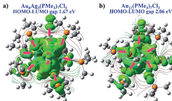
Fig. 6 DFT electron density map isocontours and HOMO–LUMO gap of (a) \text{Au}_8\text{Ag}_3(\text{PMe}_3)_7\text{Cl}_3 and (b) \text{Au}_{11}(\text{PMe}_3)_7\text{Cl}_3 from the same perspective.
