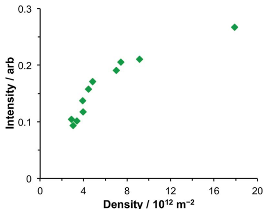
Fig. 5 Variation in the intensity of the feature at 1.43 eV in the extinction spectra of nanostructure arrays coupled to LHClI as a function of the density of nanostructures in the array.
