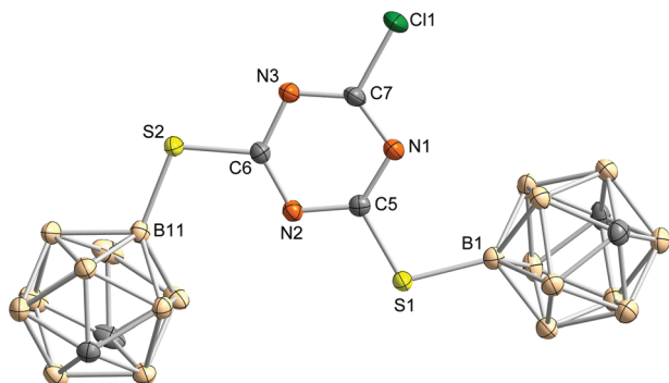
Fig. 2 Molecular structure of 2-chloro-4,6-bis(1,7-dicarbocloso-dodecaboran-9-ylthio)-1,3,5-triazine ( 3 ). Hydrogen atoms are omitted for clarity. Thermal ellipsoids are drawn at the 50% level of probability. Selected bond lengths, distances (pm) and bond angles ( ^{\circ} ): C1–C7 172.7(2), S1–C5 174.2(2), S2–C6 173.4(2), S1–B1 187.2(2), S2–B11 185.9(2), \blacklozenge ...N1 0.4, \blacklozenge ...C5 1.5, \blacklozenge ...N2 1.2, \blacklozenge ...C6 0.0, \blacklozenge ...N3 1.0, \blacklozenge ...C7 0.9, \blacklozenge ...S1 4.9, \blacklozenge ...S2 4.3, \blacklozenge ...C1 3.8, \blacklozenge ...B1 41.0, \blacklozenge ...B11 1.2; C5–S1–B1 106.1(1), C6–S2–B11 107.6(1); \blacklozenge represents the mean plane of the triazine core, formed by N1, C5, N2, C6, N3 and C7.
