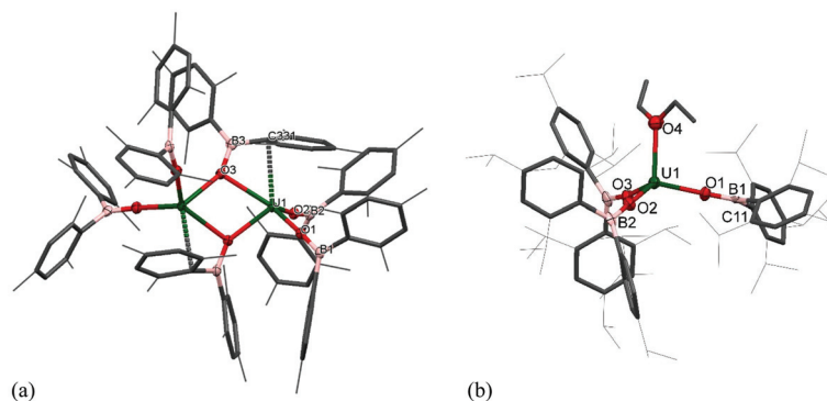
Fig. 1 Displacement ellipsoid drawing of the molecular structure of (a) \mathbf{1}^m and (b) \mathbf{1}^t\text{-Et}_2\text{O} . The hydrogen atoms are omitted and the mesityl and triisopropylphenyl groups are depicted as wireframe and capped sticks for clarity. The thermal ellipsoids are displayed at 50% probability.
