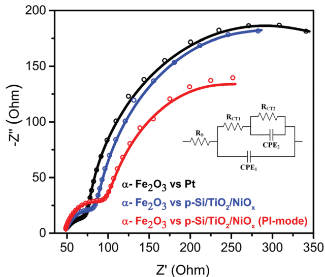
Fig. 4 Nyquist plots of \alpha - \text{Fe}_2\text{O}_3 vs. Pt or p-Si/ \text{TiO}_2 / \text{NiO}_x in 1 M NaOH (pH 13.8) under standard (1 sun) single or parallel illumination (PI-mode). The inset shows the equivalent circuit 30 employed for analyzing the Nyquist plots. The fit data are provided in ESI Table S2.†
