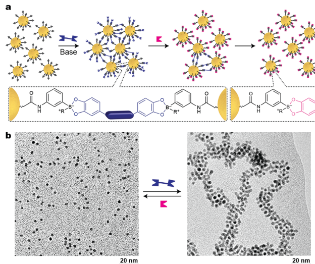
Fig. 7 Nanoparticle aggregation driven by dynamic covalent chemistry. (a) NP assembly followed by disassembly induced by a ditopic and a mono-functional boronic acid, respectively. (b) TEM images of free and covalently assembled Au NPs. Adapted with permission from ref. 45 (copyright 2016, Royal Society of Chemistry).
