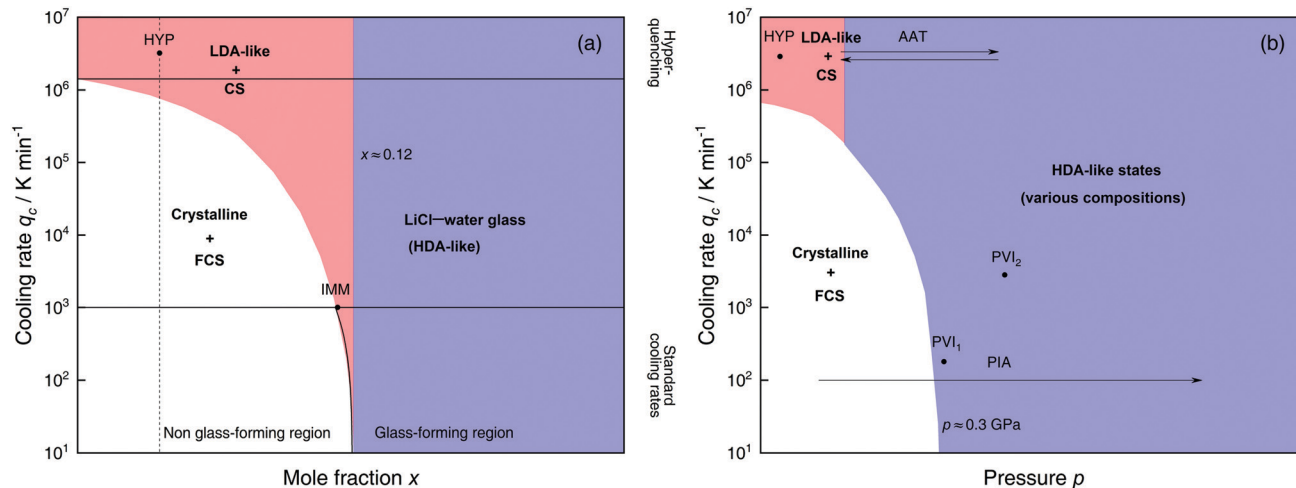
Fig. 3 Schematic diagrams indicating the final state of samples obtained after cooling LiCl–water solutions to 77 K using different mole fractions x , pressures p and cooling rates q_c . (a) Effect of q_c on solutions with different mole fraction x cooled at 1 bar. (b) Effect of q_c on dilute solutions ( x \approx 0.05 , dashed line in (a)) cooled at different pressures p . In addition, the constant temperature processes PIA and AAT are indicated by arrows. For clarity high pressure crystalline states are neglected. The white regions correspond to mixtures of ice I and freeze-concentrated glassy solution (FCS, 0.12 < x < 0.14 ). Red (or blue) regions indicate non-crystalline solutions with water in an LDA-like (or HDA-like) state. FCS and CS are characterized as HDA-like containing significant amounts of salts. Points and arrows represent experiments: ref. 130 and 131 for HYP, ref. 126 for IMM, ref. 129 for PIA, original data from the present work for AAT, ref. 132 for PVI 1 and ref. 133 and 134 for PVI 2 .
