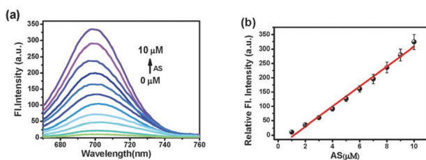
Fig. 107 (a) Fluorescence responses of 65 (2 \mu\text{M} ) to different concentrations of Angeli's salt (AS) with emission ranging from 670 to 760 nm. \lambda_{\text{ex}} = 690 nm. (b) Relationship between the relative fluorescence intensity at 700 nm and concentrations of AS (0, 1, 2, 3, 4, 5, 6, 7, 8, 9, 10 \mu\text{M} ). Fluorescence spectra were acquired in HEPES buffer solution (10 mM, 0.5% DMSO, 0.5% TW 80, pH 5.0). Copyright 2014 Royal Society of Chemistry.
