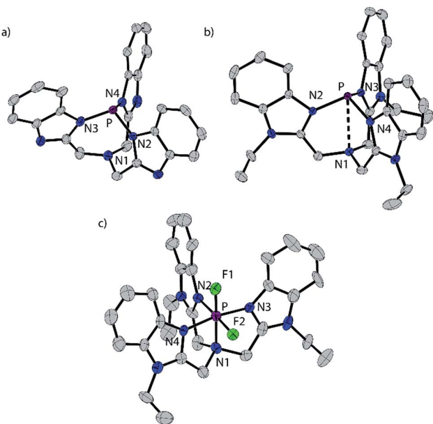
Fig. 1 Solid state structures of one of two independent molecules of P(BIM) (a), the cation in [\text{P}(\text{BIMe}_3)]^{3+} \cdot (\text{MeCN})_2 (b), and cation in [\text{PF}_2(\text{BIMe}_3)]^{3+} \cdot \text{MeCN} (c). Thermal ellipsoids are shown at a 50% probability level. Hydrogen atoms, solvent molecules and triflate anions are omitted for clarity. Inter-atomic distances and angles are summarized in Table 2.
