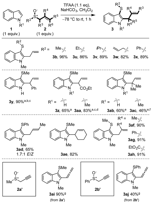
Scheme 3 Exploring the scope of the allylic sulfonide in the dual functionalisation cascade of indoles. a The corresponding E -allylic sulfonides were used ( i.e. \text{R}^6 = \text{H} ). b \text{3y}/\text{4y} = 4.8 : 1 . c Yield determined by ^1\text{H-NMR} . d \text{3aa}/\text{4aa} = 3 : 1 . e Heated at 60\text{ }^\circ\text{C} , 30 min. f \text{3ac}/\text{4ac} = 3.3 : 1 . g Heated at 60\text{ }^\circ\text{C} , 1 h. Regioisomer ratios determined from ^1\text{H-NMR} spectra of the crude reaction mixture.
