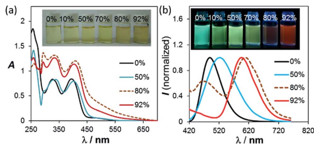
Fig. 4 (a) Changes in the absorption and (b) fluorescence spectra of BO-1 in THF ( 1 \times 10^{-4} M), with increasing water content. For the complete spectra, see ESI † .
