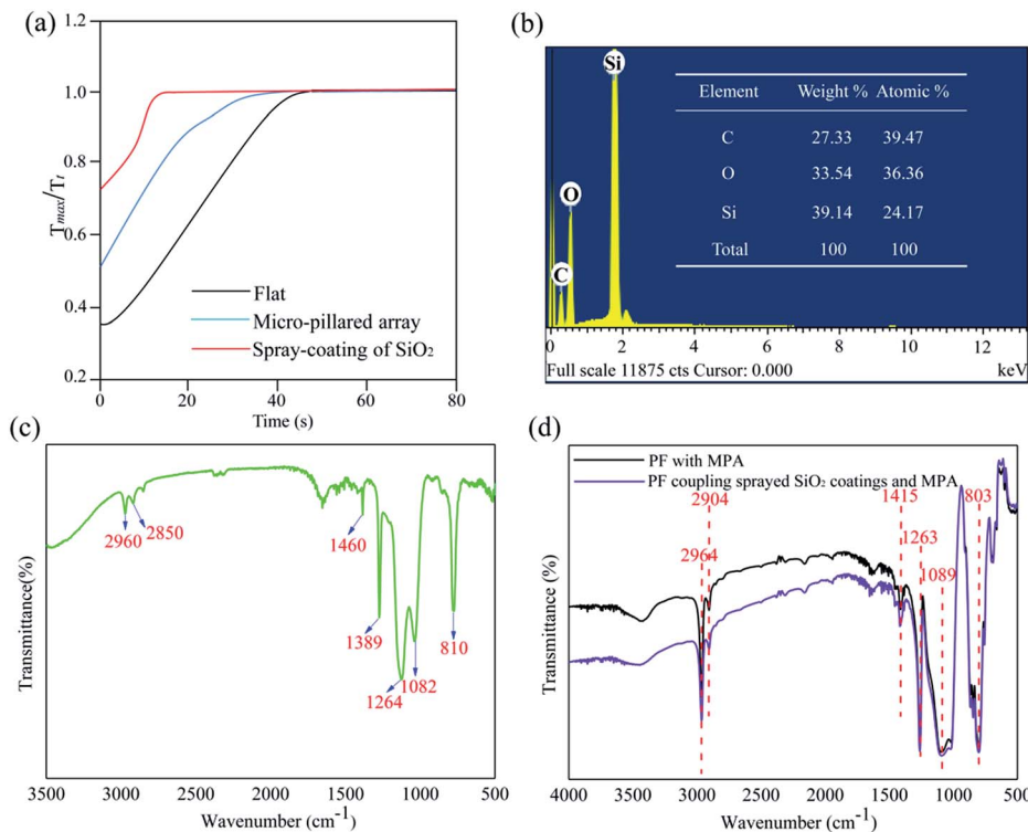
Fig. 5 (a) Antifogging of the three PFs is quantified by performing time-lapse transmittance measurements ( T_f ) to determine the required time to restore their original optical properties ( T_{max} ). The PF coupled with sprayed SiO 2 coatings and the MPA shows a significantly faster recovery from fogging. (b) Energy-dispersive X-ray spectroscopy (EDS) spectra of the PF coupled sprayed SiO 2 coatings and the MPA. (c) FTIR spectra of the commercial SiO 2 coating agent. (d) FTIR spectra of the PF with the MPA (black) and the PF coupled with sprayed SiO 2 coatings and the MPA (purple).
