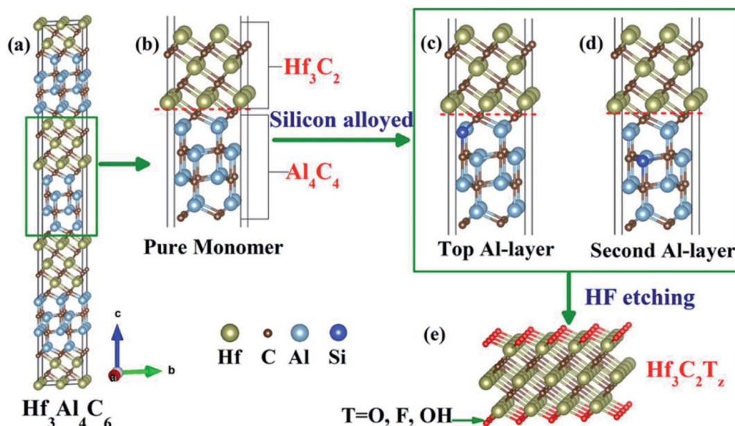
Fig. 2 Schematic illustration of the synthesis of Hf 3 C 2 T z MXene from nanolaminated phase Hf 3 [Al(Si)] 4 C 6 . (a) Structure of Hf 3 Al 4 C 6 , (b) structure of pure Hf 3 Al 4 C 6 monomer, (c) and (d) structure of two Hf 3 Al 4 C 6 monomers with different silicon alloying, and (e) side view of Hf 3 C 2 MXene. Reprinted with permission of ref. 36 Copyright 2017 American Chemical Society.
